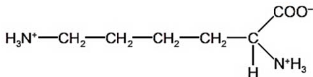
lysine
